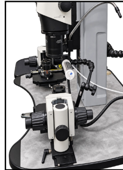
STAGE or CROSS-BEAM MOUNT articulated arm attachment LCF3-LEDKIT-AA-R2
