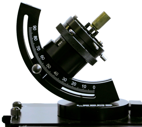
.40-caliber casing held by the extraction groove for viewing extractor marks
