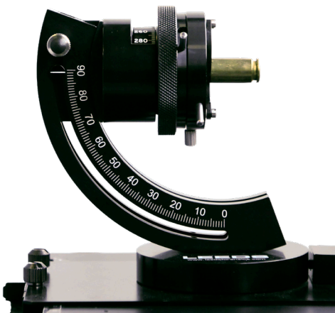
.40-caliber casing held by the inside diameter for viewing chambermarks
